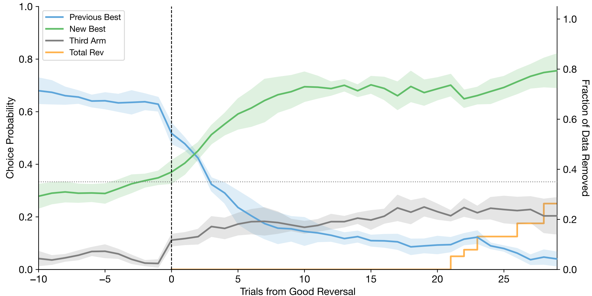
Good Reversal-Aligned Choices (mean \pm se across subjects | n=5 subjects, n=38 reversals)
